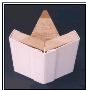
Solid Wood Mullion
