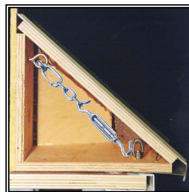
Hanging System can be used in conjunction with Bay/Bow Pre-Fabricated Roof.
